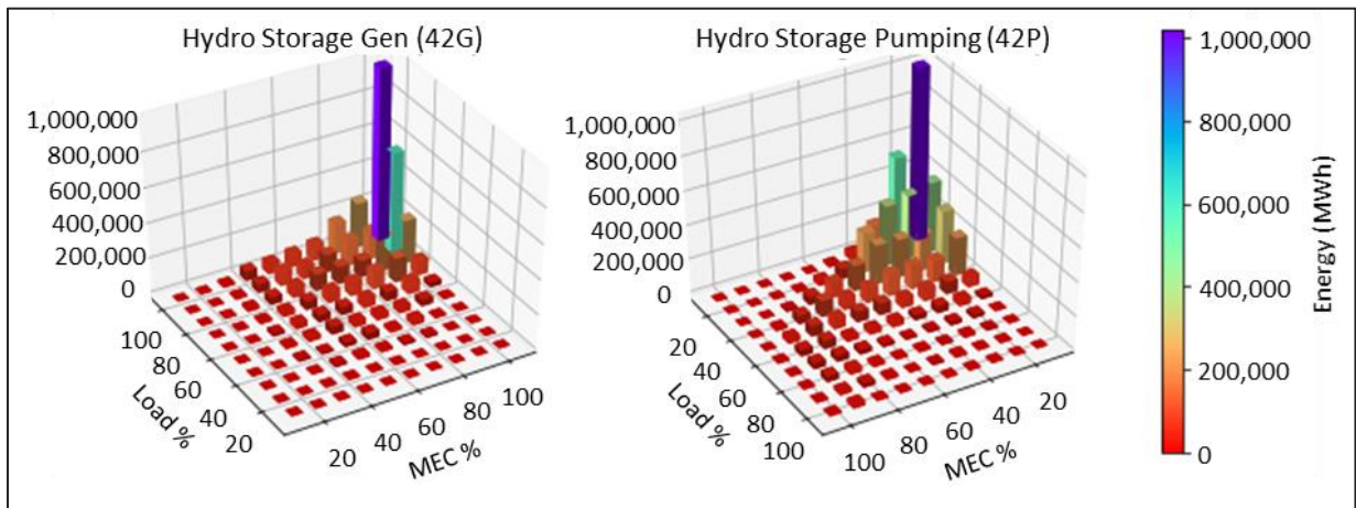
Figure 2-8. Comparison of PSH operations in pumping vs. generation modes in MISO (2015–2017). Marginal Energy Charge (MEC) is the energy component of the LMP. (Data source: MISO)
