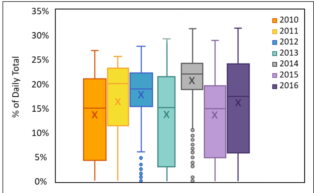
Figure 2-14. Percentage of spinning reserve provided by conventional hydropower resources in MISO. Hydropower’s total capacity ranges from 3–5% of total the installed generation capacity. (Data source: MISO)
